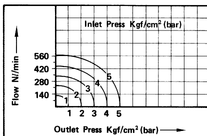
● 流體：空氣 ADS-20
