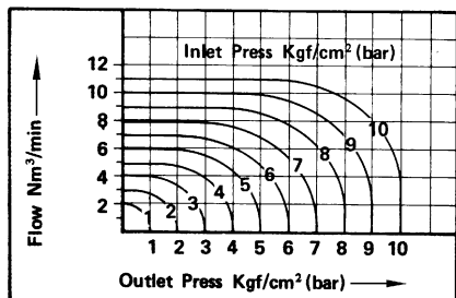
● 流體：空氣 ADS-35.40(AF)
