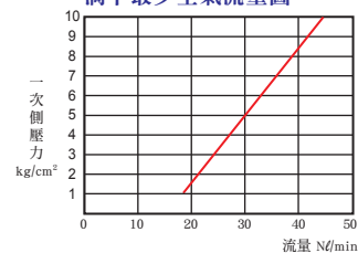
滴下最少空氣流量圖
