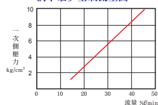
滴下最少空氣流量圖
